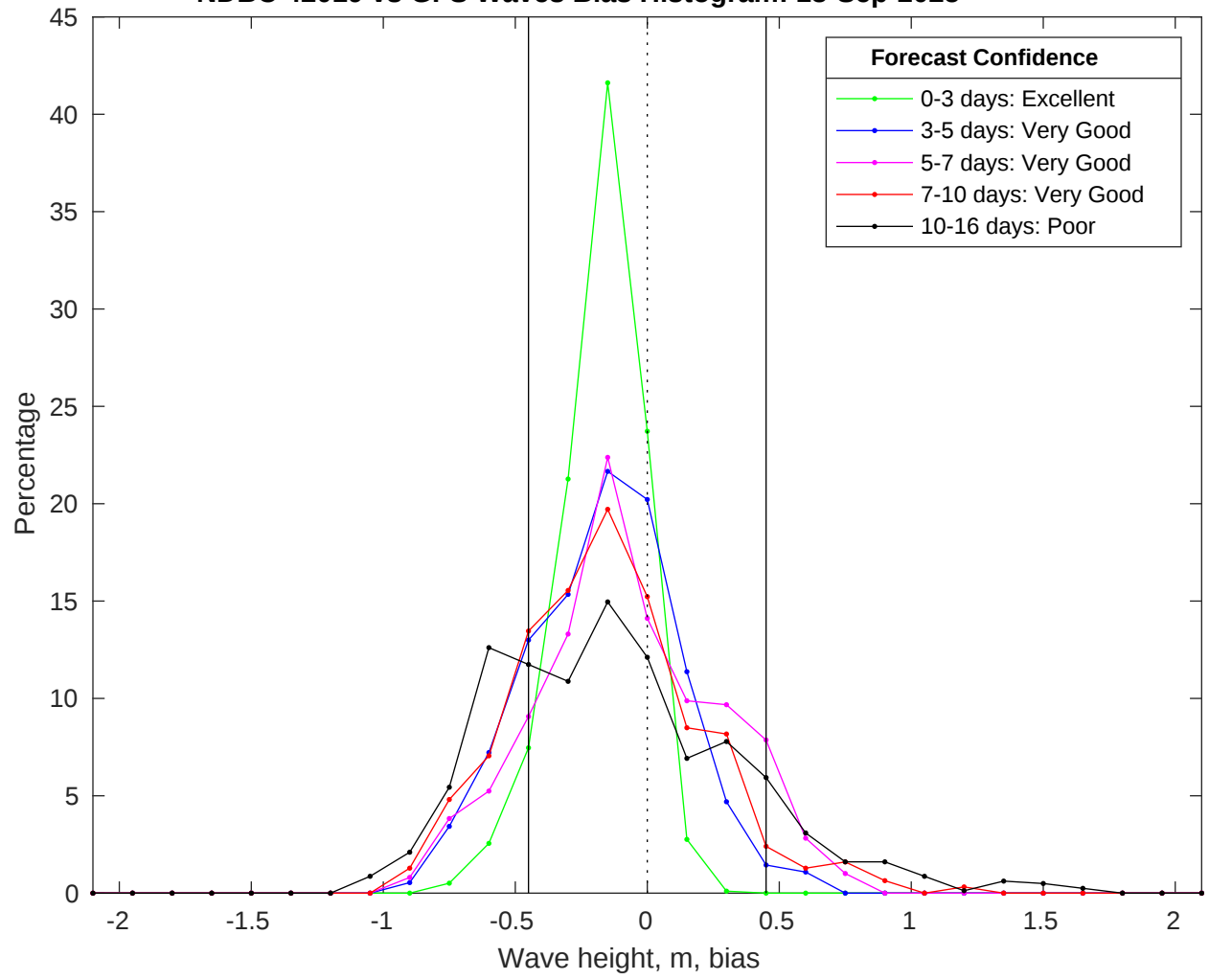
NDBC 42019 vs GFS Waves Bias Histogram: 18-Sep-2025
