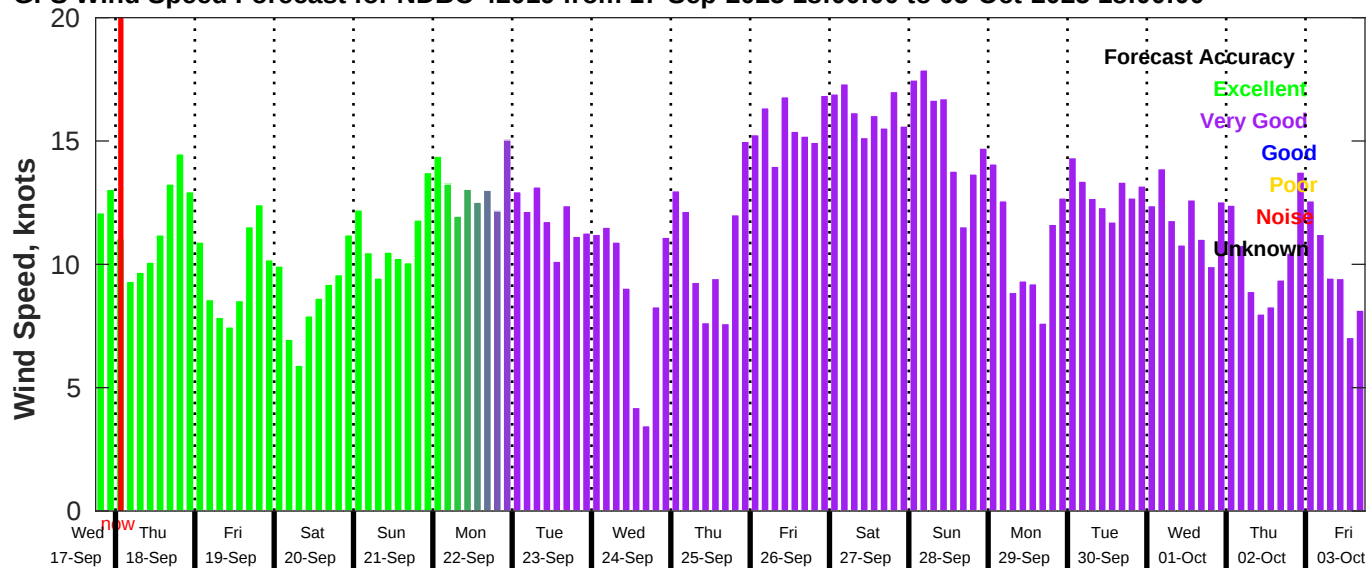
GFS Wind Speed Forecast for NDBC 42019 from 17-Sep-2025 18:00:00 to 03-Oct-2025 18:00:00
