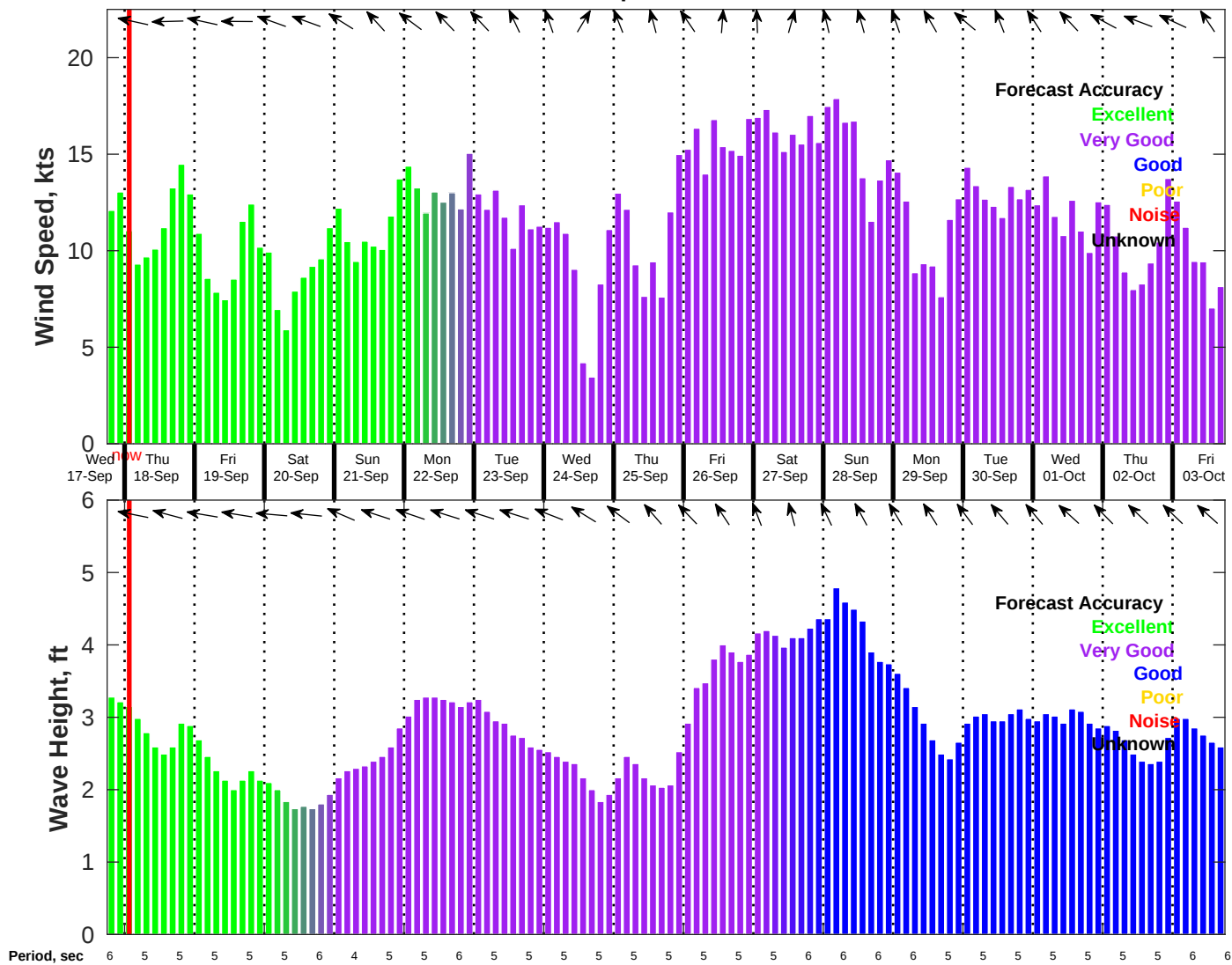
Wind & Wave Forecast for NDBC 42019 from 17-Sep-2025 18:00:00 to 03-Oct-2025 18:00:00
