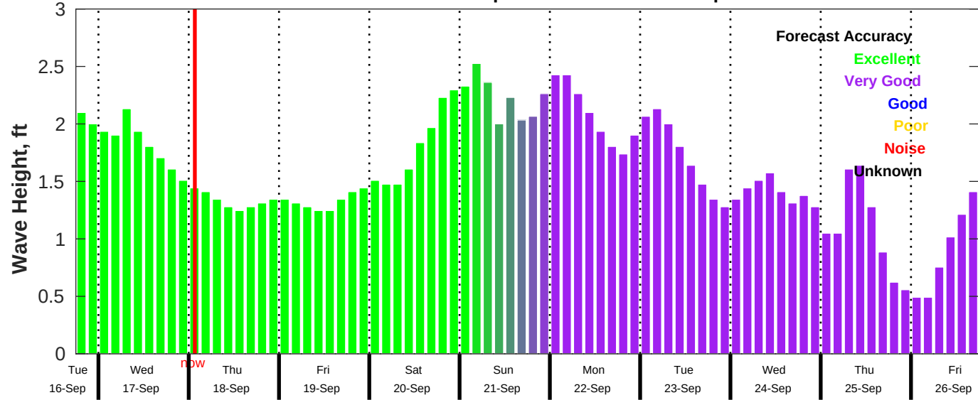
CMEMS Wave Forecast for NDBC 42035 from 16-Sep-2025 18:00:00 to 26-Sep-2025 18:00:00
