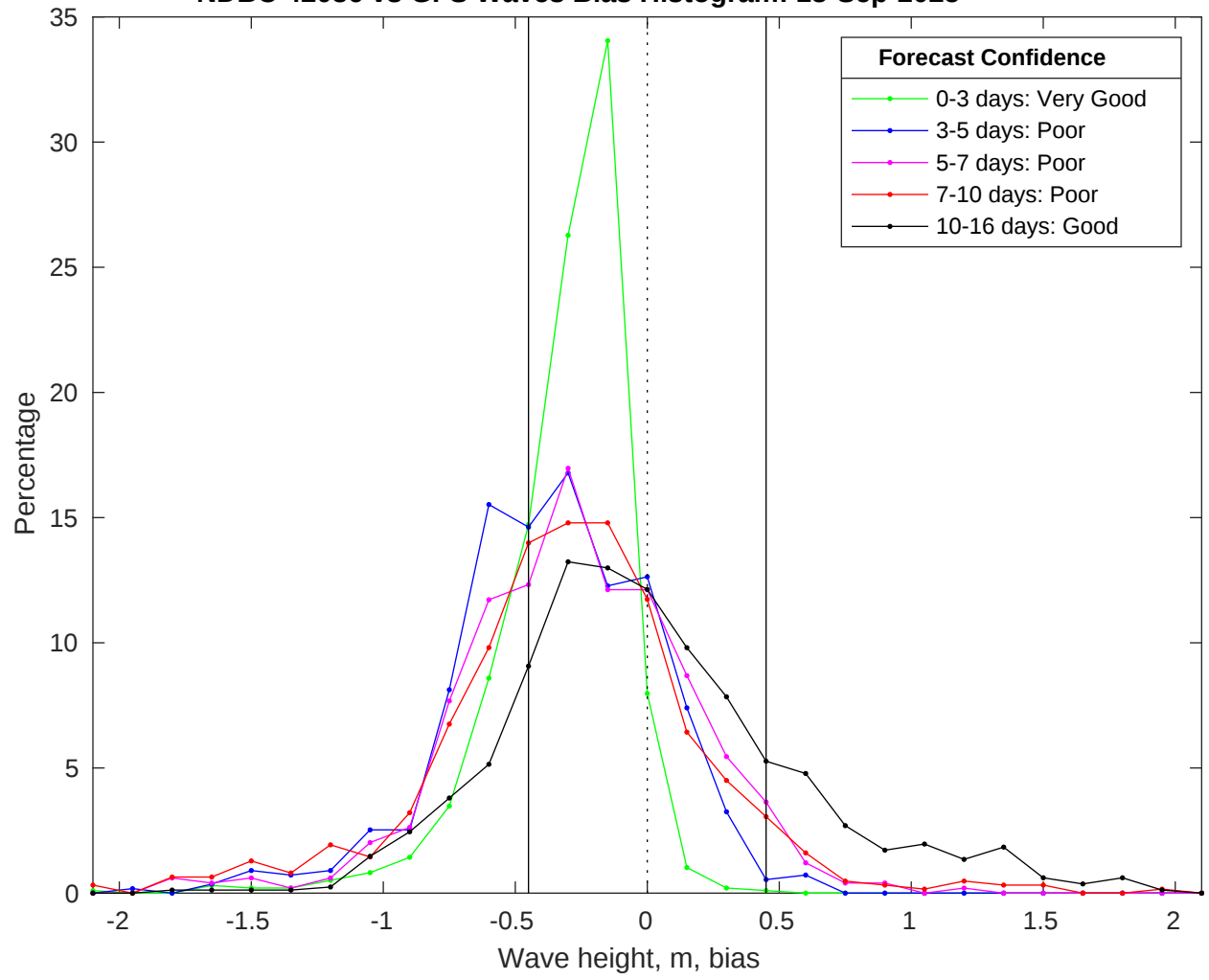
NDBC 42036 vs GFS Waves Bias Histogram: 18-Sep-2025
