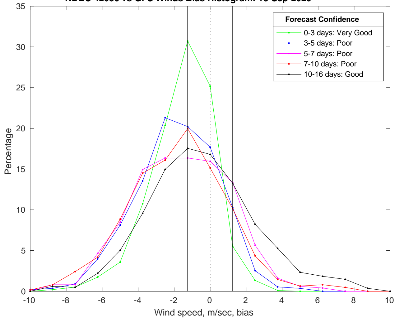
NDBC 42036 vs GFS Winds Bias Histogram: 18-Sep-2025
