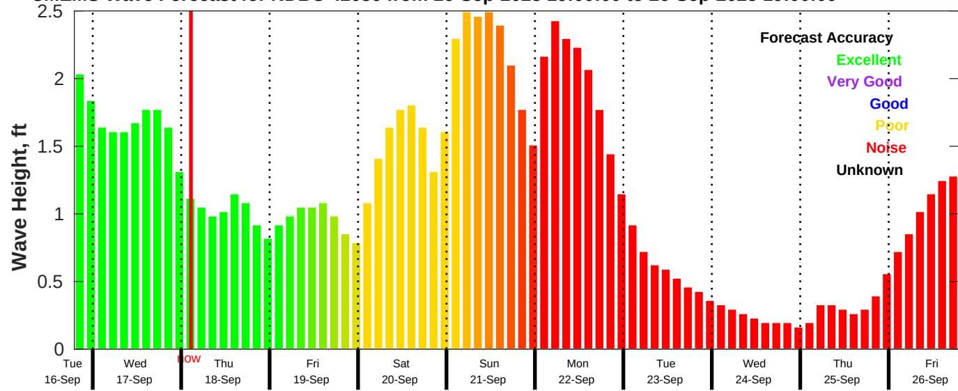
CMEMS Wave Forecast for NDBC 42036 from 16-Sep-2025 19:00:00 to 26-Sep-2025 19:00:00
