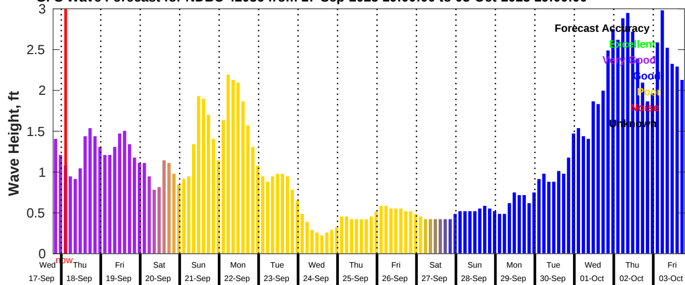
GFS Wave Forecast for NDBC 42036 from 17-Sep-2025 19:00:00 to 03-Oct-2025 19:00:00
