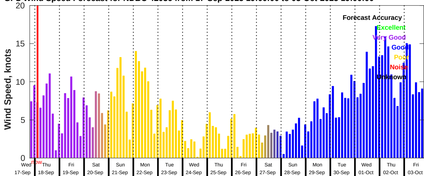
GFS Wind Speed Forecast for NDBC 42036 from 17-Sep-2025 19:00:00 to 03-Oct-2025 19:00:00
