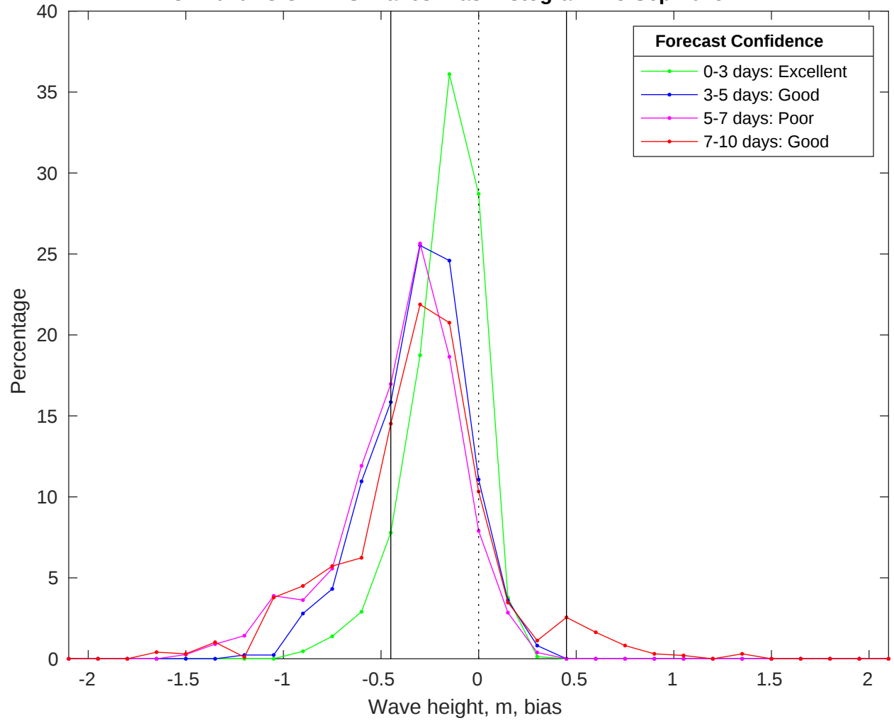
NDBC 42040 vs CMEMS Waves Bias Histogram: 18-Sep-2025
