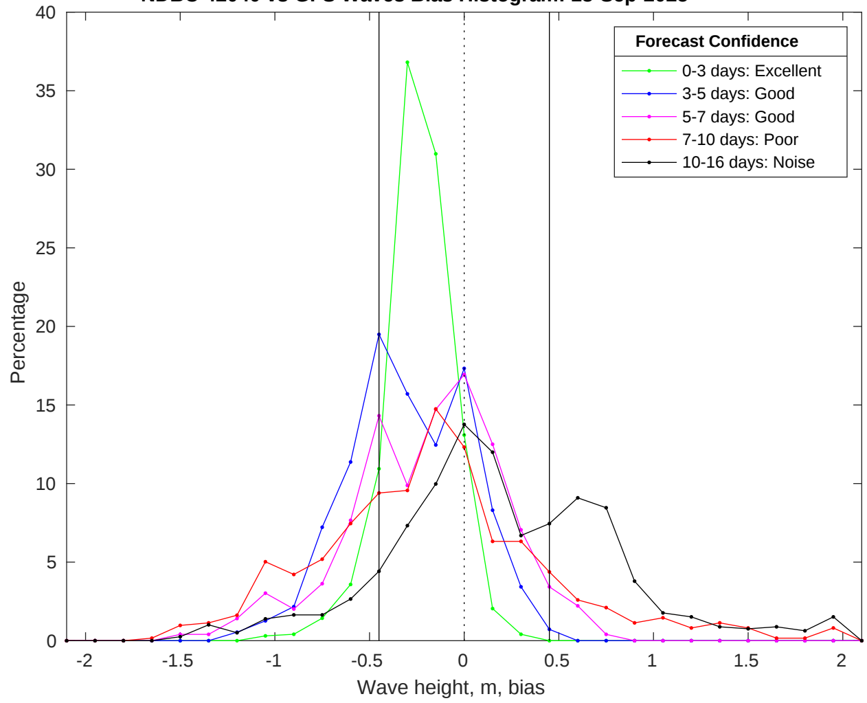
NDBC 42040 vs GFS Waves Bias Histogram: 18-Sep-2025
