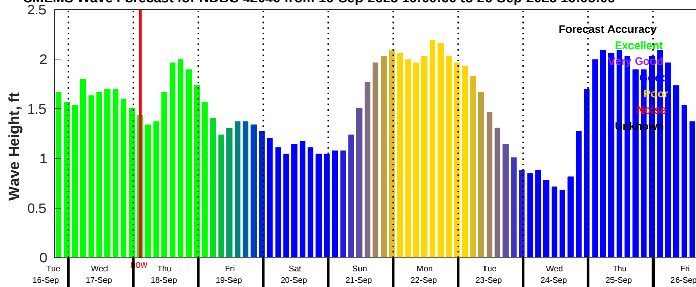
CMEMS Wave Forecast for NDBC 42040 from 16-Sep-2025 19:00:00 to 26-Sep-2025 19:00:00
