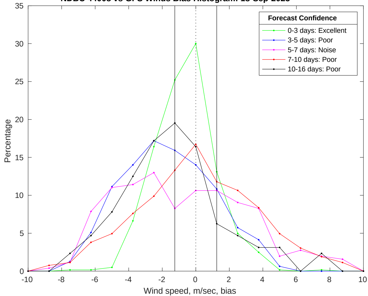
NDBC 44008 vs GFS Winds Bias Histogram: 18-Sep-2025
