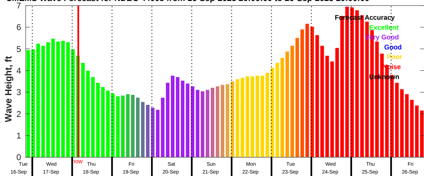
CMEMS Wave Forecast for NDBC 44008 from 16-Sep-2025 20:00:00 to 26-Sep-2025 20:00:00
