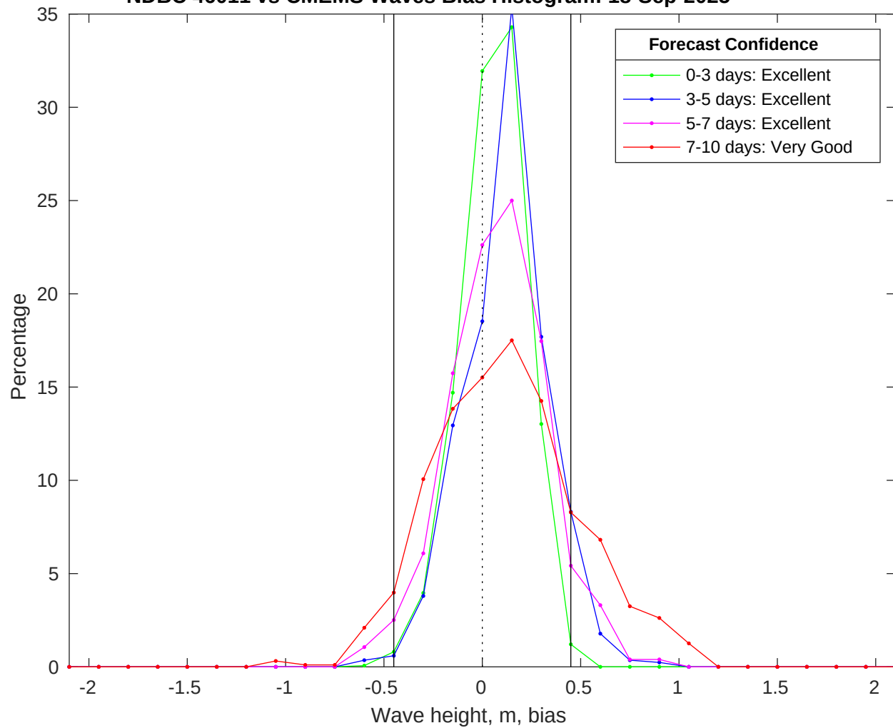
NDBC 46011 vs CMEMS Waves Bias Histogram: 18-Sep-2025
