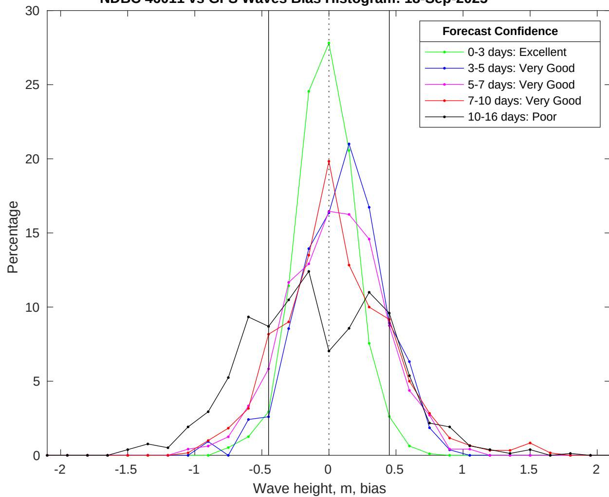
NDBC 46011 vs GFS Waves Bias Histogram: 18-Sep-2025
