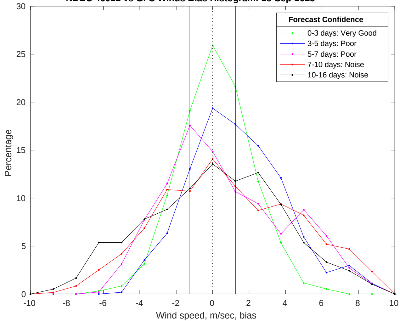
NDBC 46011 vs GFS Winds Bias Histogram: 18-Sep-2025
