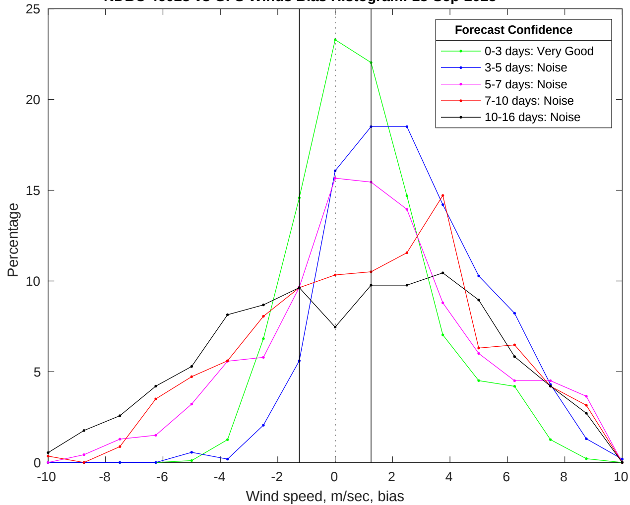
NDBC 46028 vs GFS Winds Bias Histogram: 18-Sep-2025
