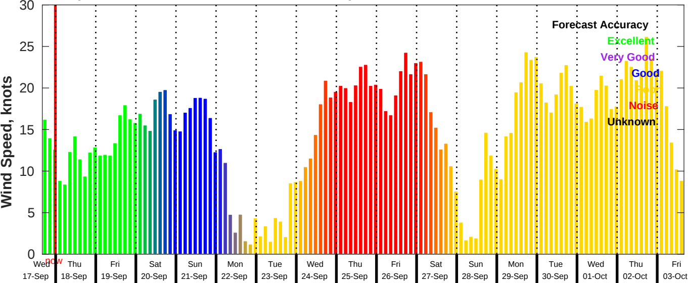
GFS Wind Speed Forecast for NDBC 46054 from 17-Sep-2025 16:00:00 to 03-Oct-2025 16:00:00
