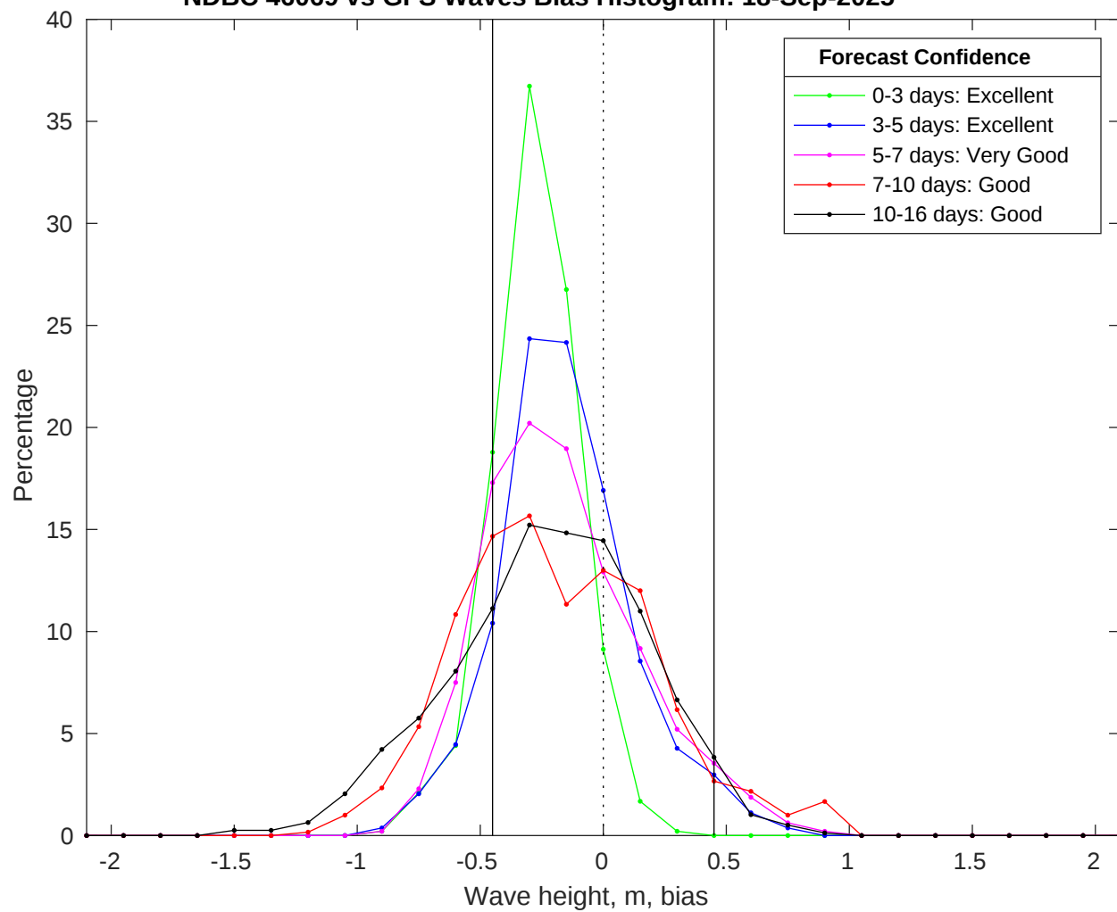
NDBC 46069 vs GFS Waves Bias Histogram: 18-Sep-2025
