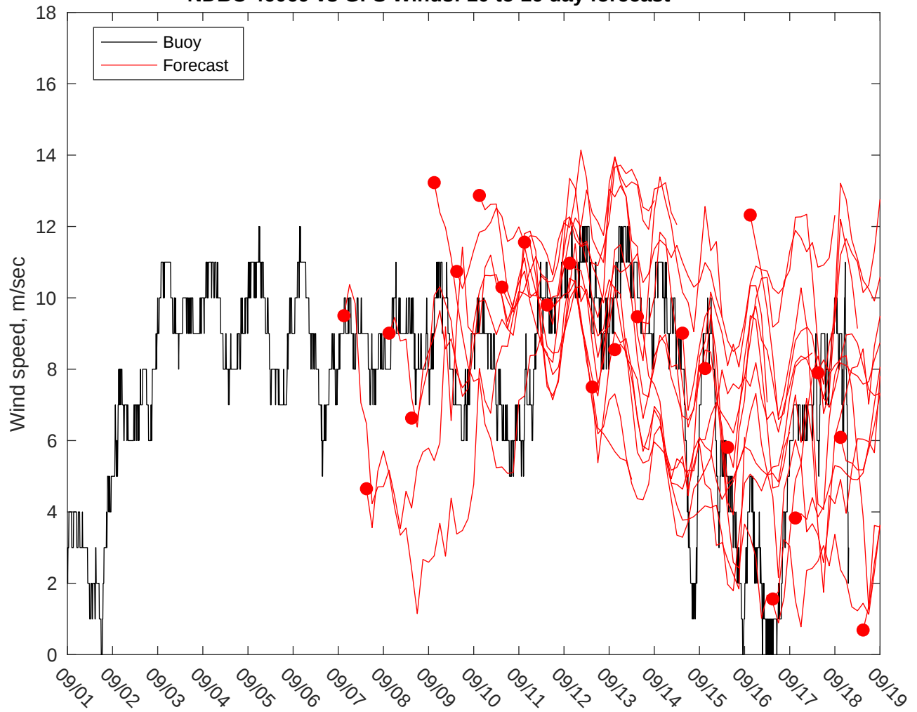
NDBC 46069 vs GFS Winds: 10 to 16 day forecast
