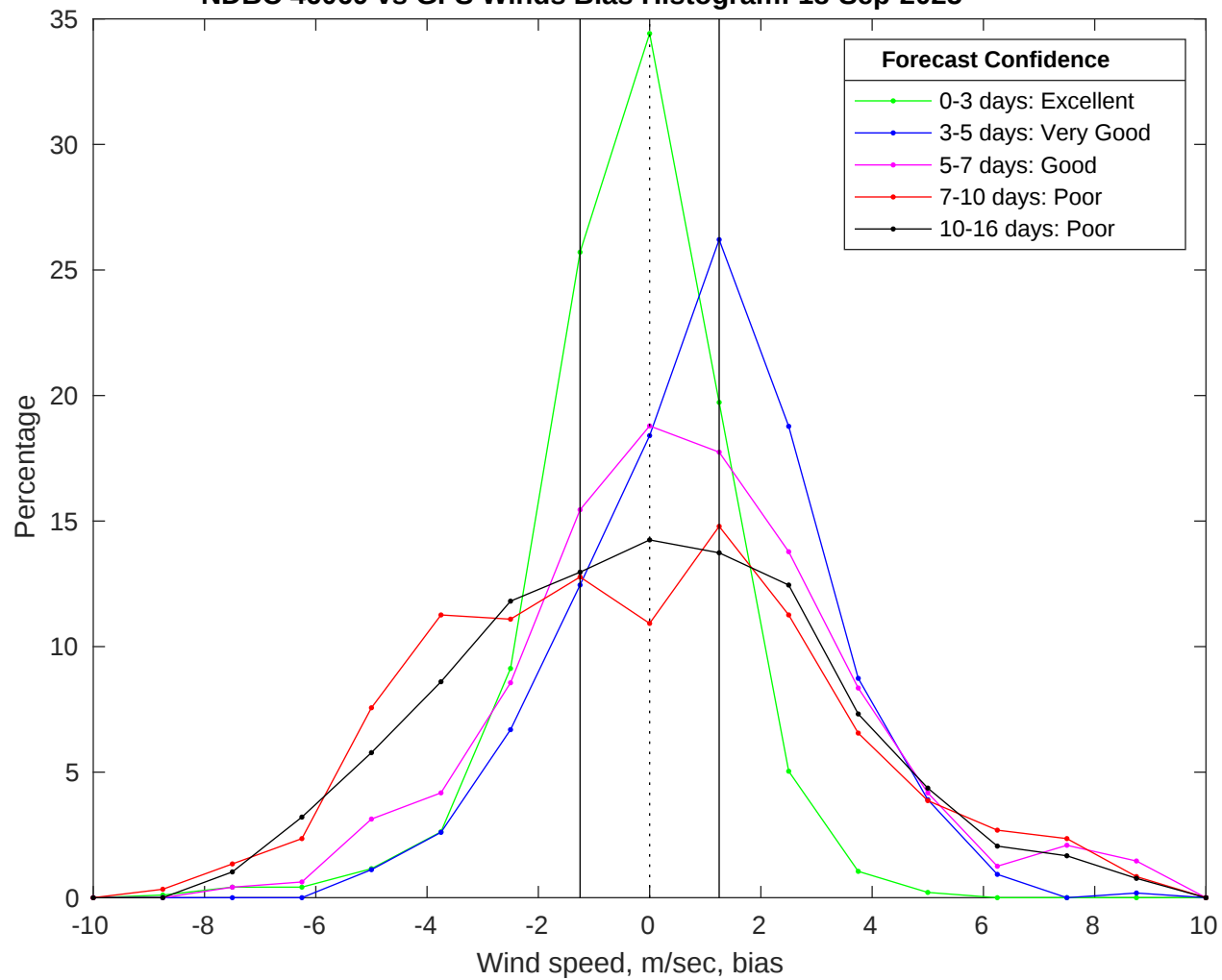
NDBC 46069 vs GFS Winds Bias Histogram: 18-Sep-2025
