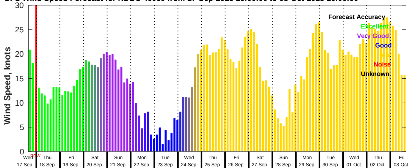
GFS Wind Speed Forecast for NDBC 46069 from 17-Sep-2025 16:00:00 to 03-Oct-2025 16:00:00
