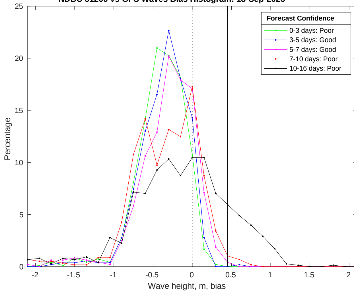
NDBC 51209 vs GFS Waves Bias Histogram: 18-Sep-2025
