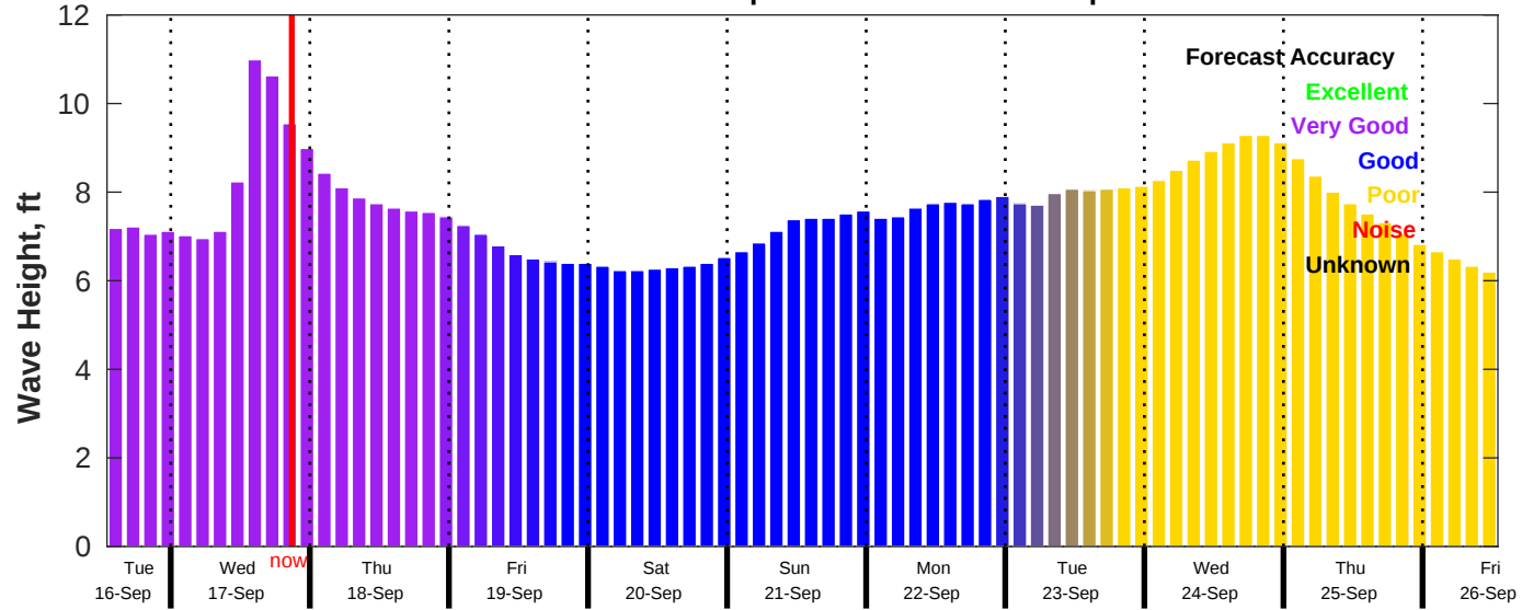
CMEMS Wave Forecast for NDBC 51209 from 16-Sep-2025 13:00:00 to 26-Sep-2025 13:00:00
