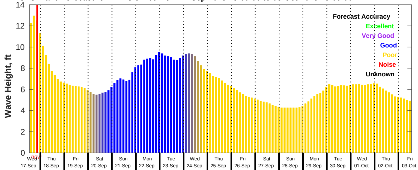
GFS Wave Forecast for NDBC 51209 from 17-Sep-2025 13:00:00 to 03-Oct-2025 13:00:00
