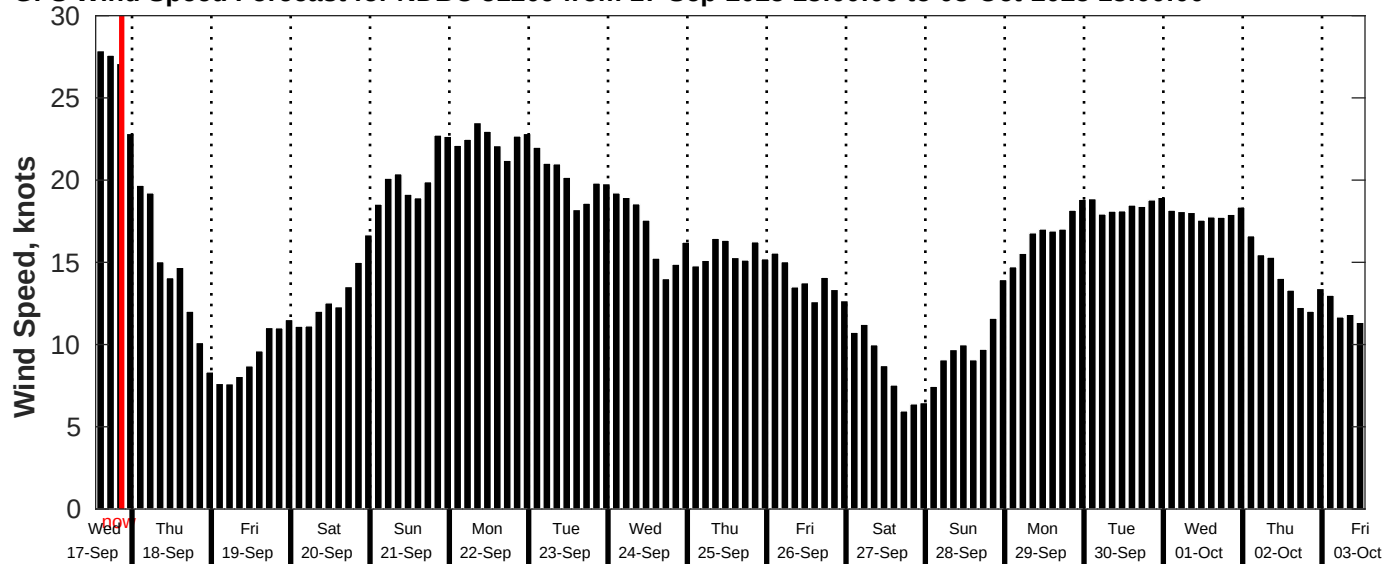
GFS Wind Speed Forecast for NDBC 51209 from 17-Sep-2025 13:00:00 to 03-Oct-2025 13:00:00
