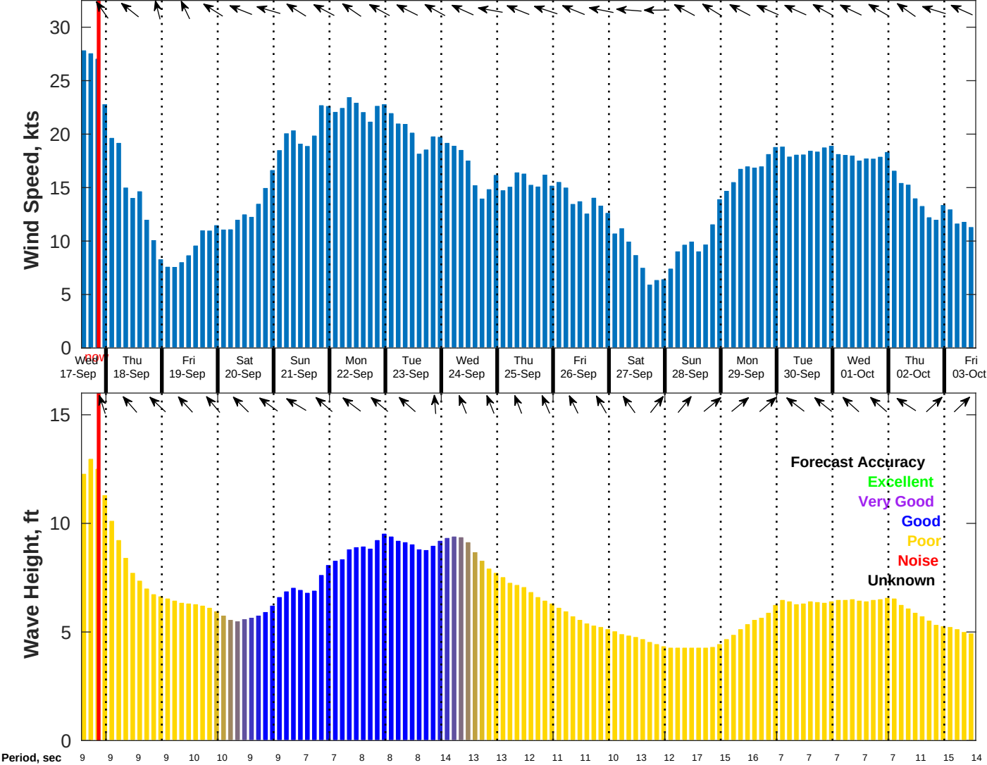
Wind & Wave Forecast for NDBC 51209 from 17-Sep-2025 13:00:00 to 03-Oct-2025 13:00:00
