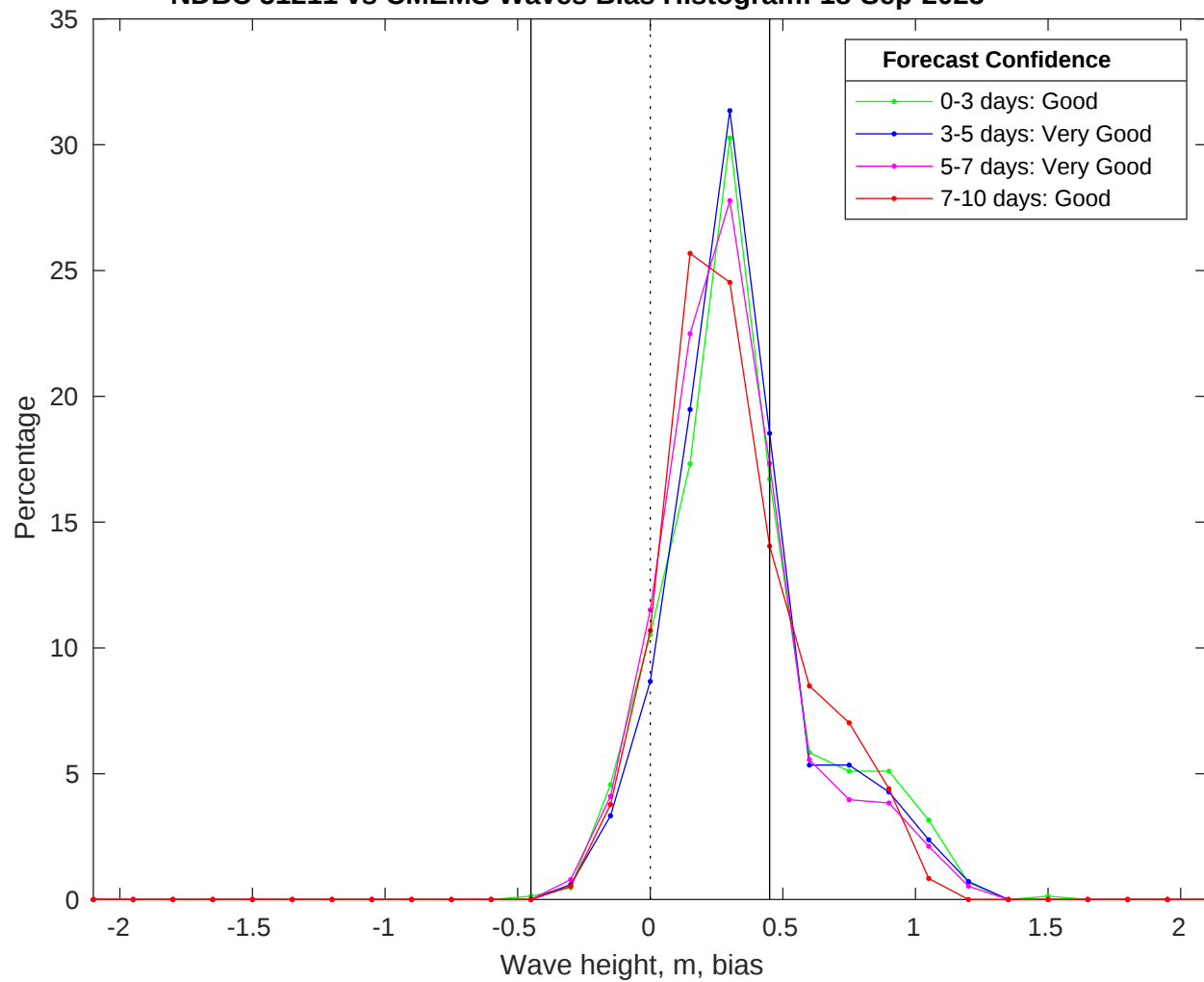
NDBC 51211 vs CMEMS Waves Bias Histogram: 18-Sep-2025
