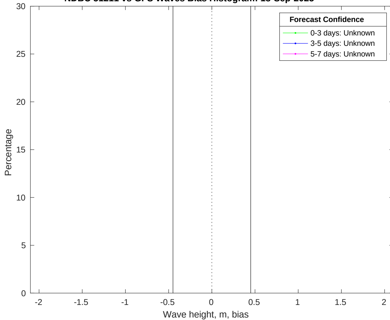
NDBC 51211 vs GFS Waves Bias Histogram: 18-Sep-2025
