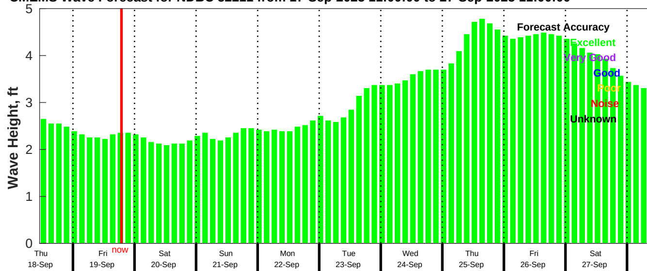
CMEMS Wave Forecast for NDBC 52211 from 17-Sep-2025 11:00:00 to 27-Sep-2025 11:00:00
