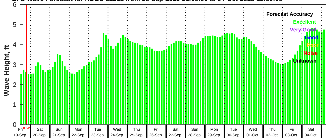
GFS Wave Forecast for NDBC 52211 from 18-Sep-2025 11:00:00 to 04-Oct-2025 11:00:00
