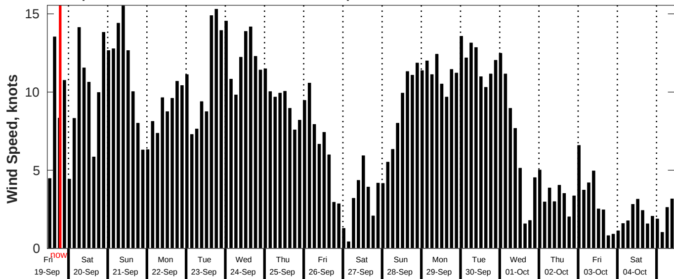
GFS Wind Speed Forecast for NDBC 52211 from 18-Sep-2025 11:00:00 to 04-Oct-2025 11:00:00
