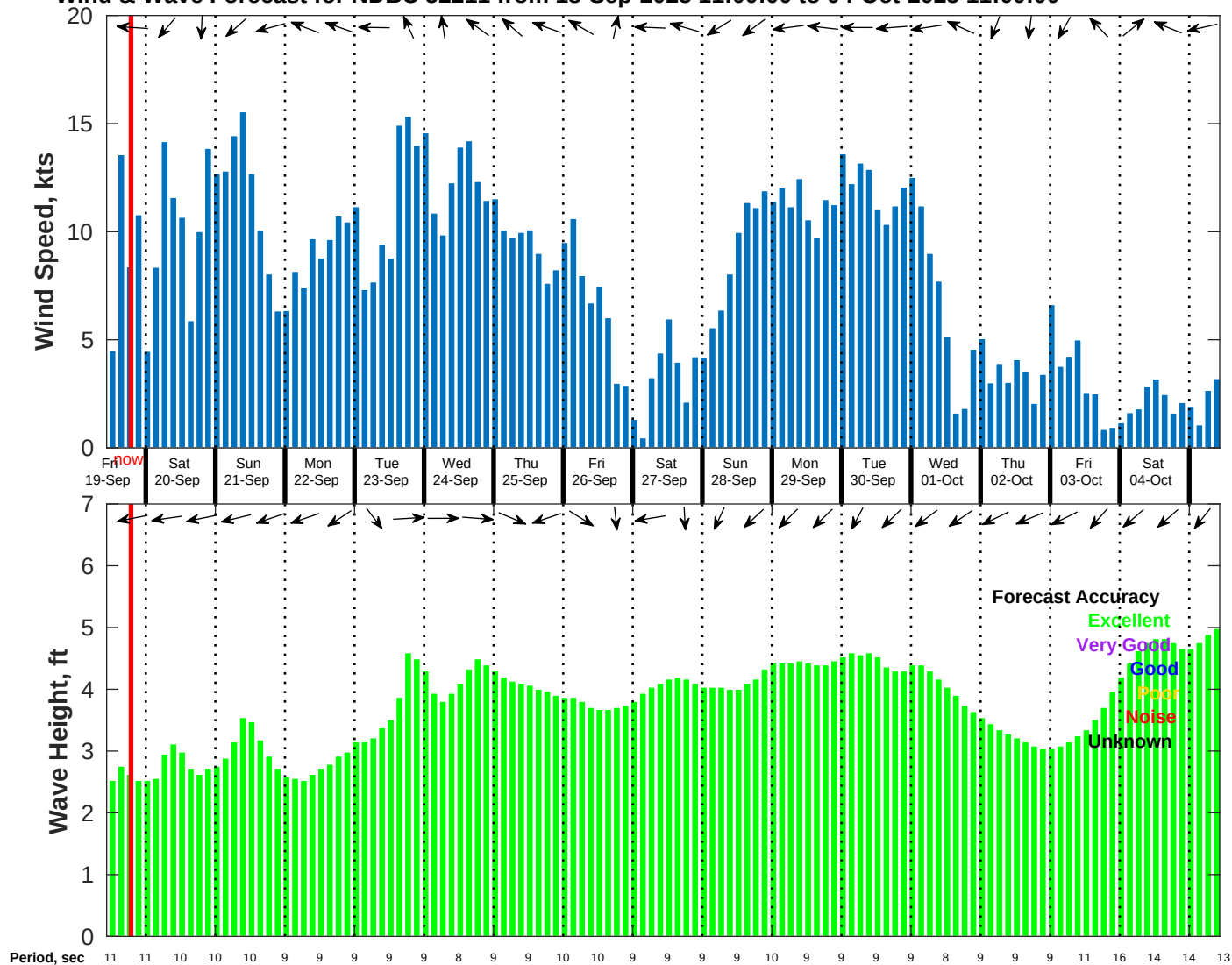
Wind & Wave Forecast for NDBC 52211 from 18-Sep-2025 11:00:00 to 04-Oct-2025 11:00:00
