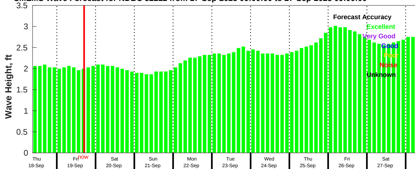
CMEMS Wave Forecast for NDBC 52212 from 17-Sep-2025 09:00:00 to 27-Sep-2025 09:00:00
