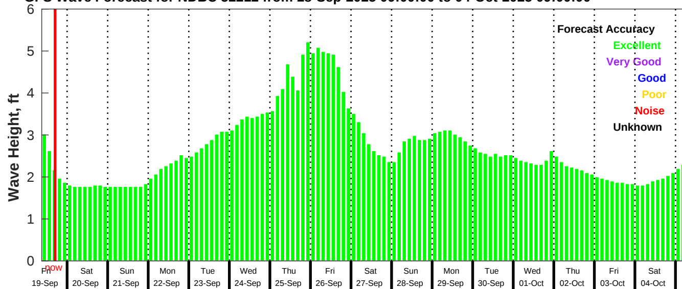
GFS Wave Forecast for NDBC 52212 from 18-Sep-2025 09:00:00 to 04-Oct-2025 09:00:00
