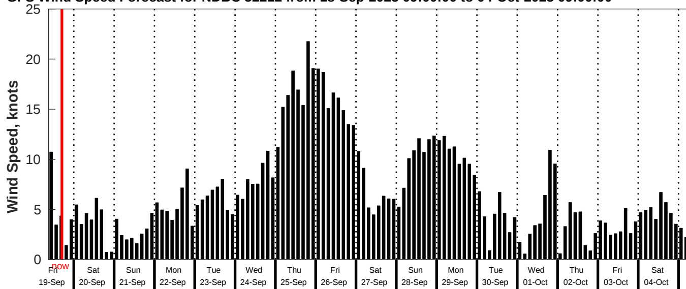
GFS Wind Speed Forecast for NDBC 52212 from 18-Sep-2025 09:00:00 to 04-Oct-2025 09:00:00
