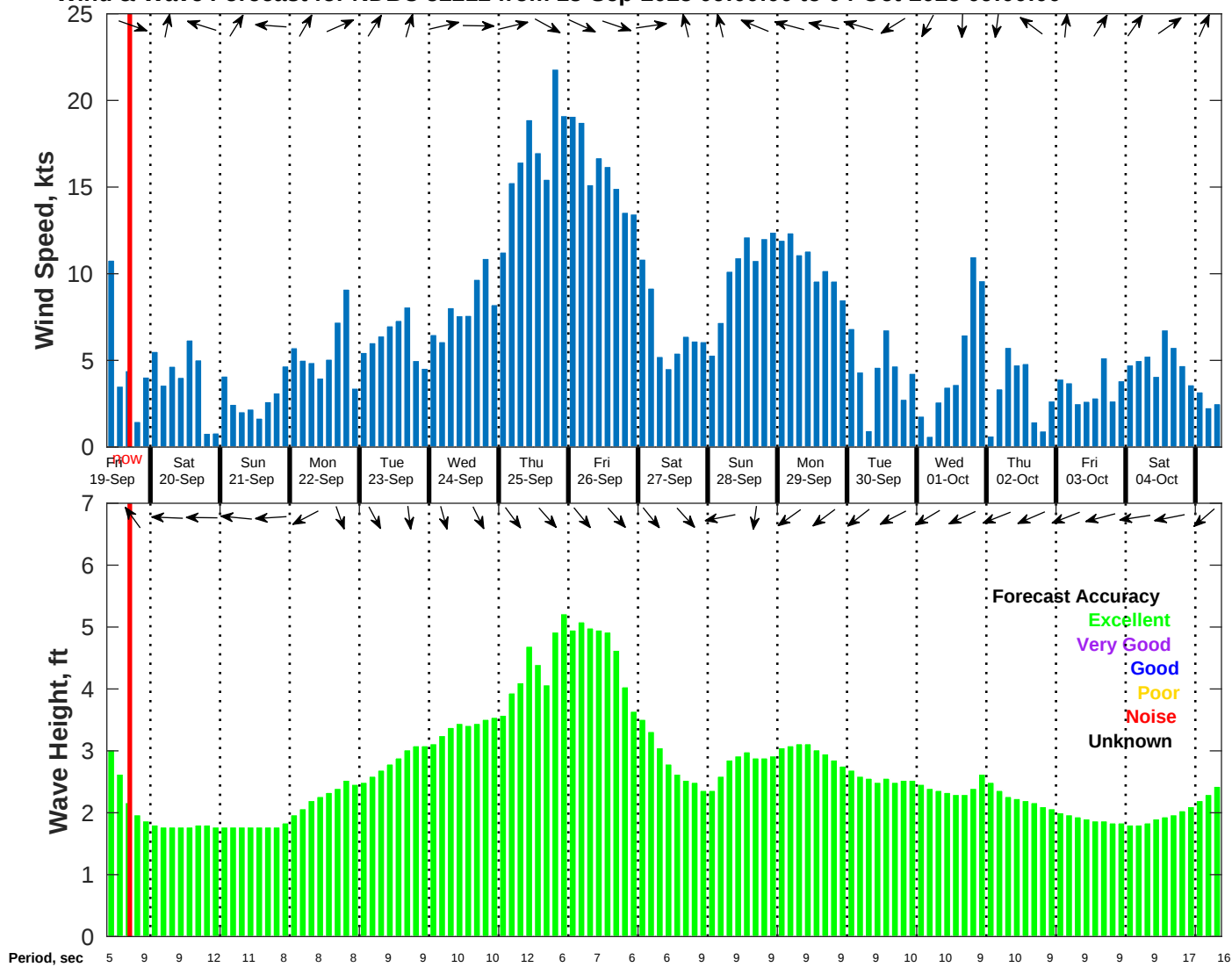
Wind & Wave Forecast for NDBC 52212 from 18-Sep-2025 09:00:00 to 04-Oct-2025 09:00:00
