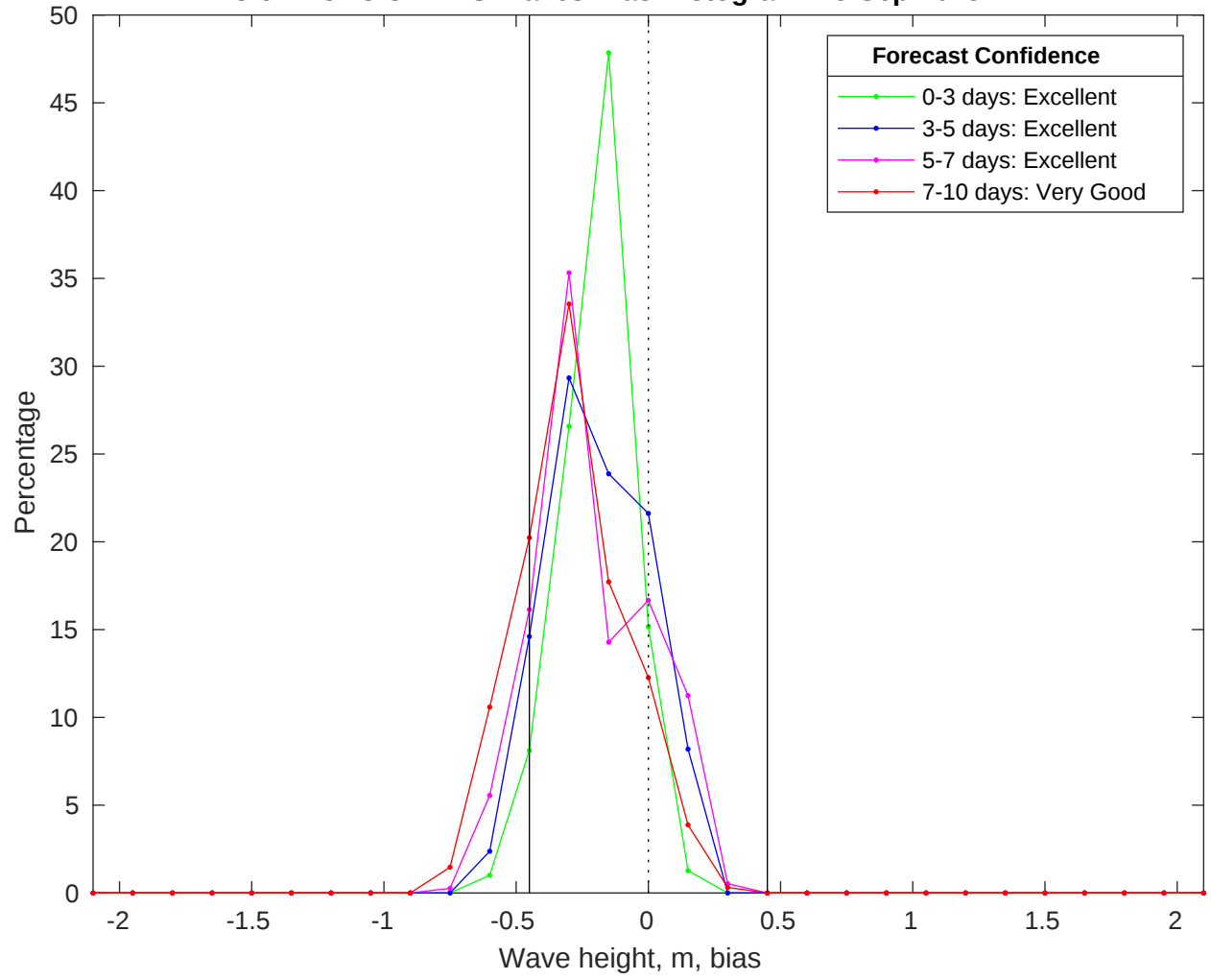
NDBC 52213 vs CMEMS Waves Bias Histogram: 18-Sep-2025
