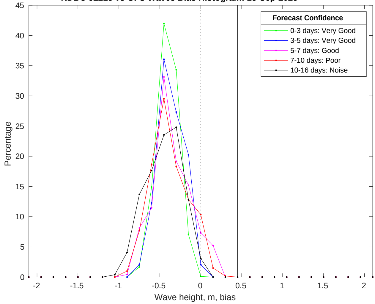
NDBC 52213 vs GFS Waves Bias Histogram: 18-Sep-2025
