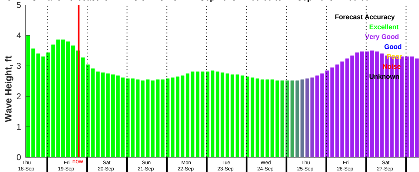
CMEMS Wave Forecast for NDBC 52213 from 17-Sep-2025 11:00:00 to 27-Sep-2025 11:00:00
