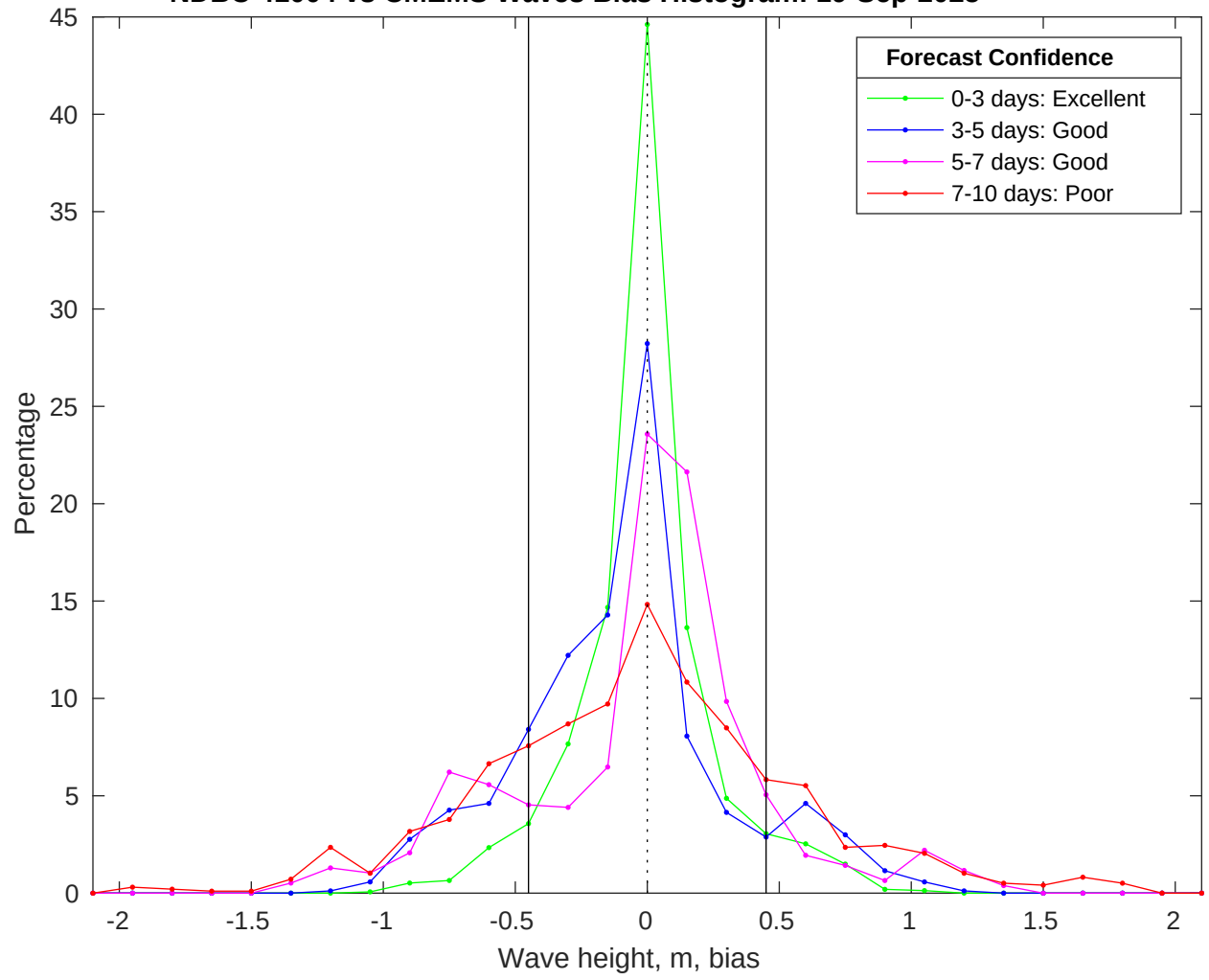
NDBC 41004 vs CMEMS Waves Bias Histogram: 19-Sep-2025
