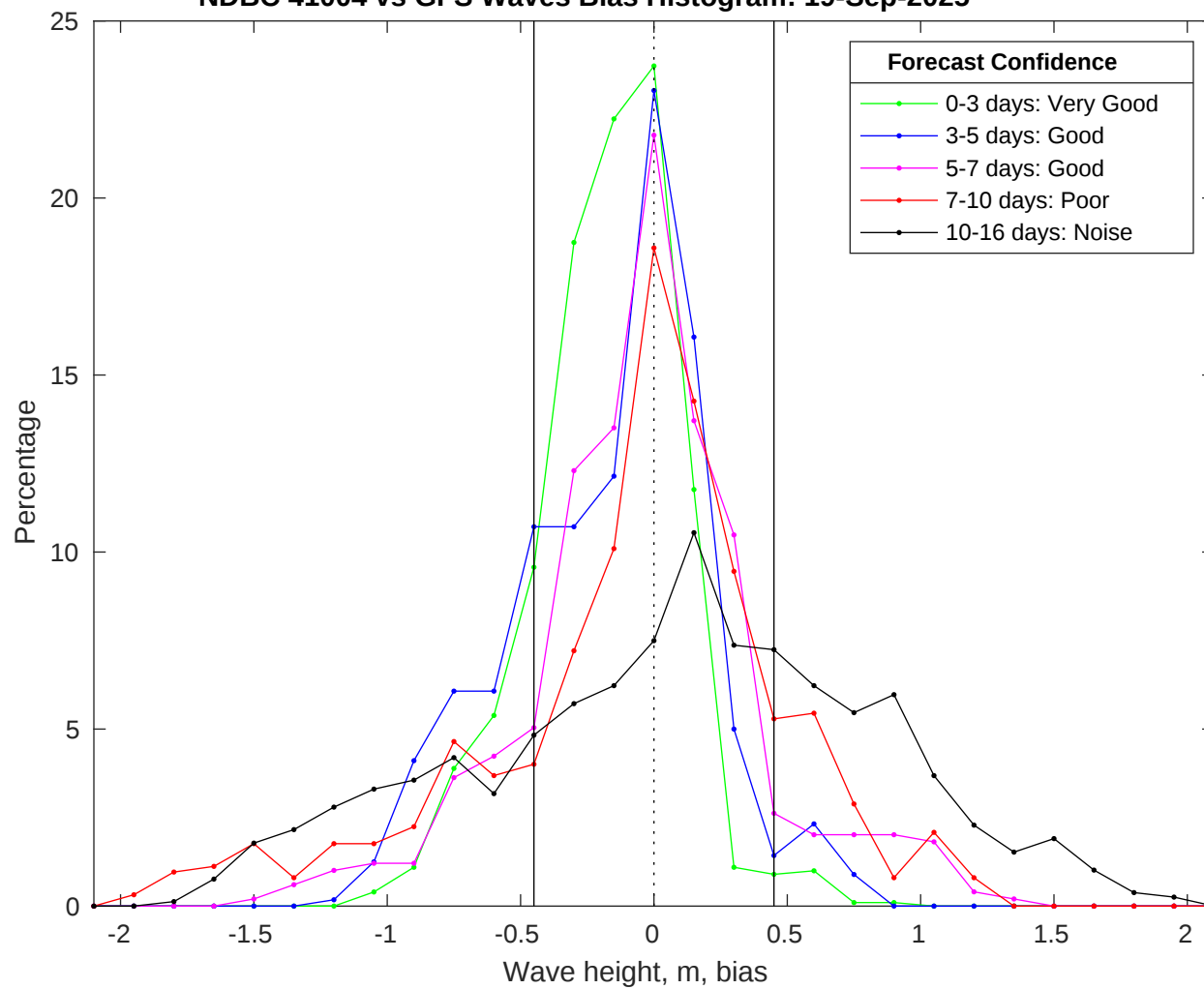
NDBC 41004 vs GFS Waves Bias Histogram: 19-Sep-2025
