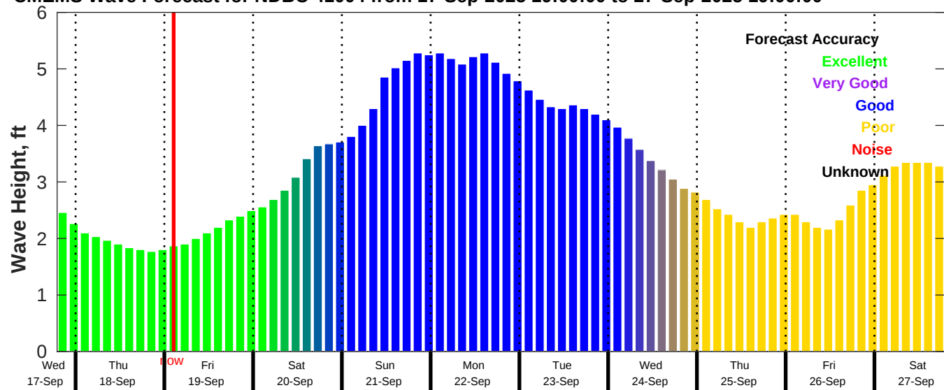
CMEMS Wave Forecast for NDBC 41004 from 17-Sep-2025 19:00:00 to 27-Sep-2025 19:00:00
