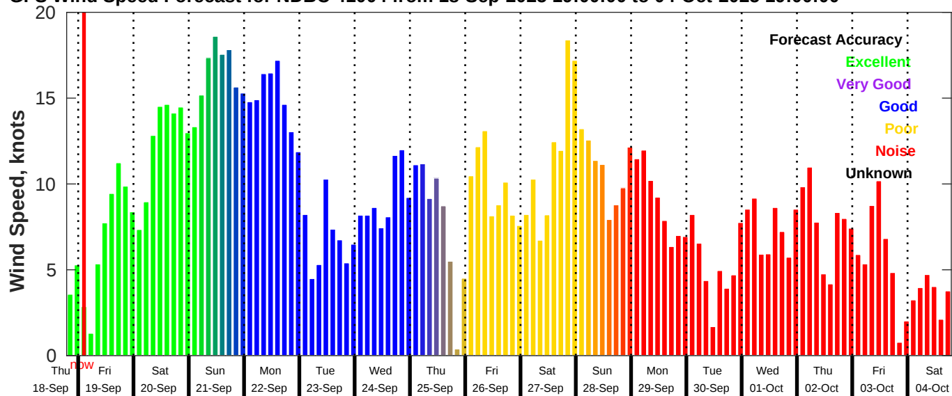
GFS Wind Speed Forecast for NDBC 41004 from 18-Sep-2025 19:00:00 to 04-Oct-2025 19:00:00
