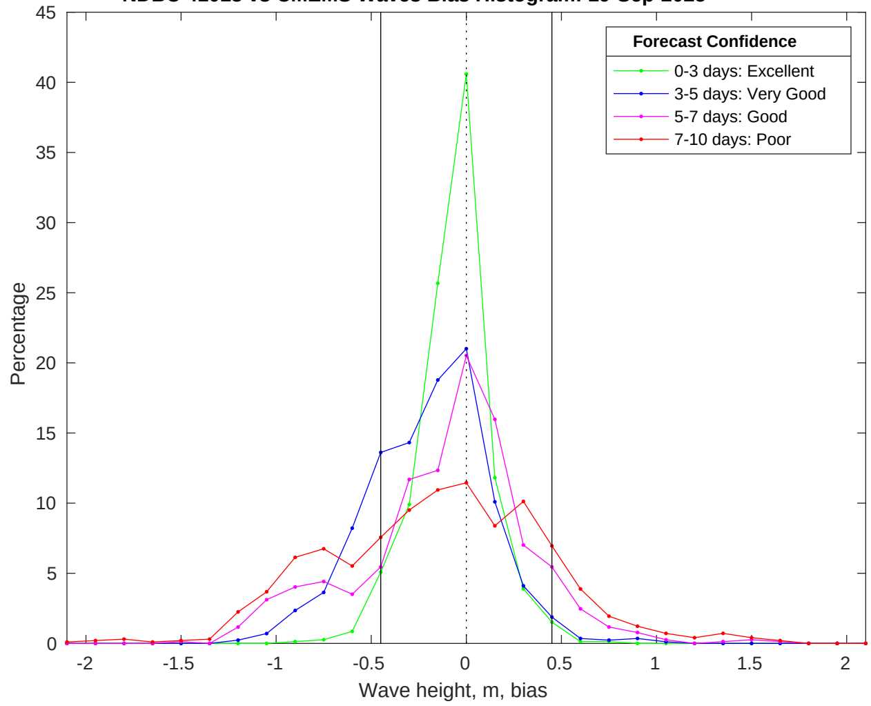
NDBC 41013 vs CMEMS Waves Bias Histogram: 19-Sep-2025
