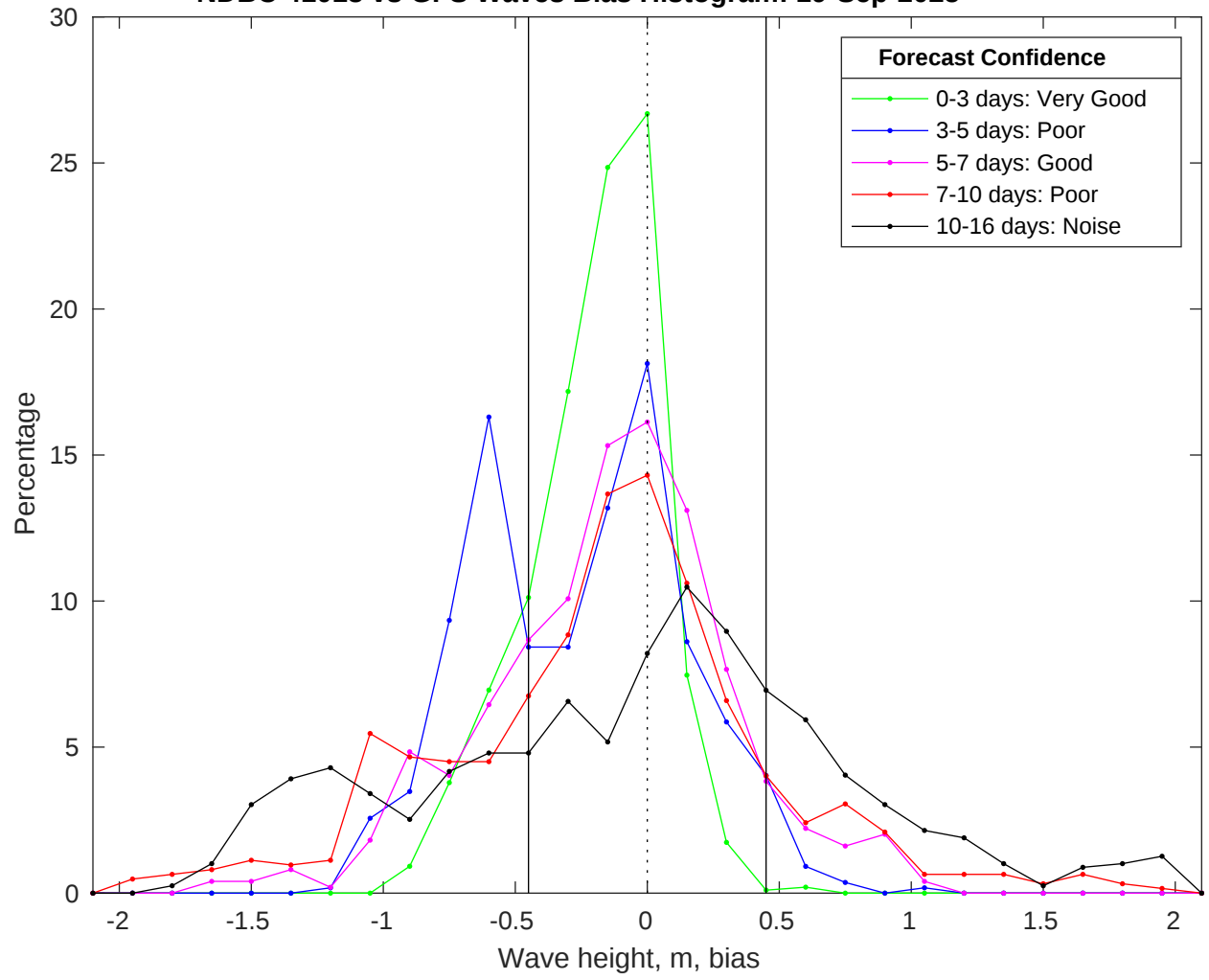
NDBC 41013 vs GFS Waves Bias Histogram: 19-Sep-2025
