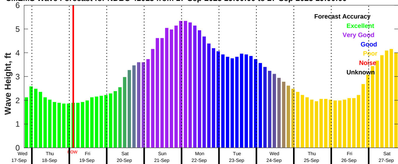
CMEMS Wave Forecast for NDBC 41013 from 17-Sep-2025 19:00:00 to 27-Sep-2025 19:00:00
