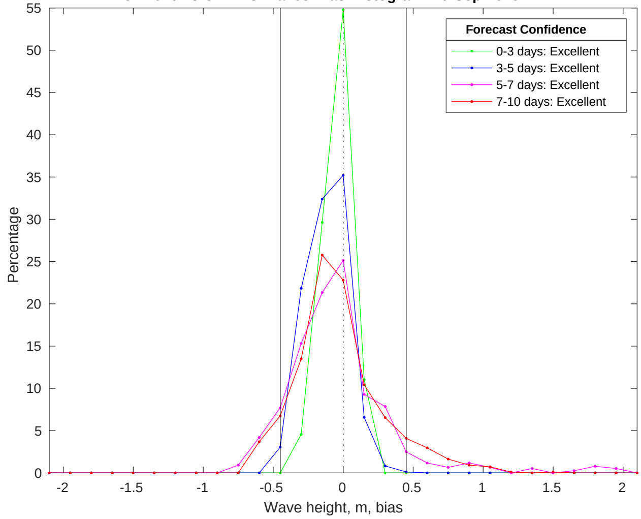
NDBC 41040 vs CMEMS Waves Bias Histogram: 19-Sep-2025
