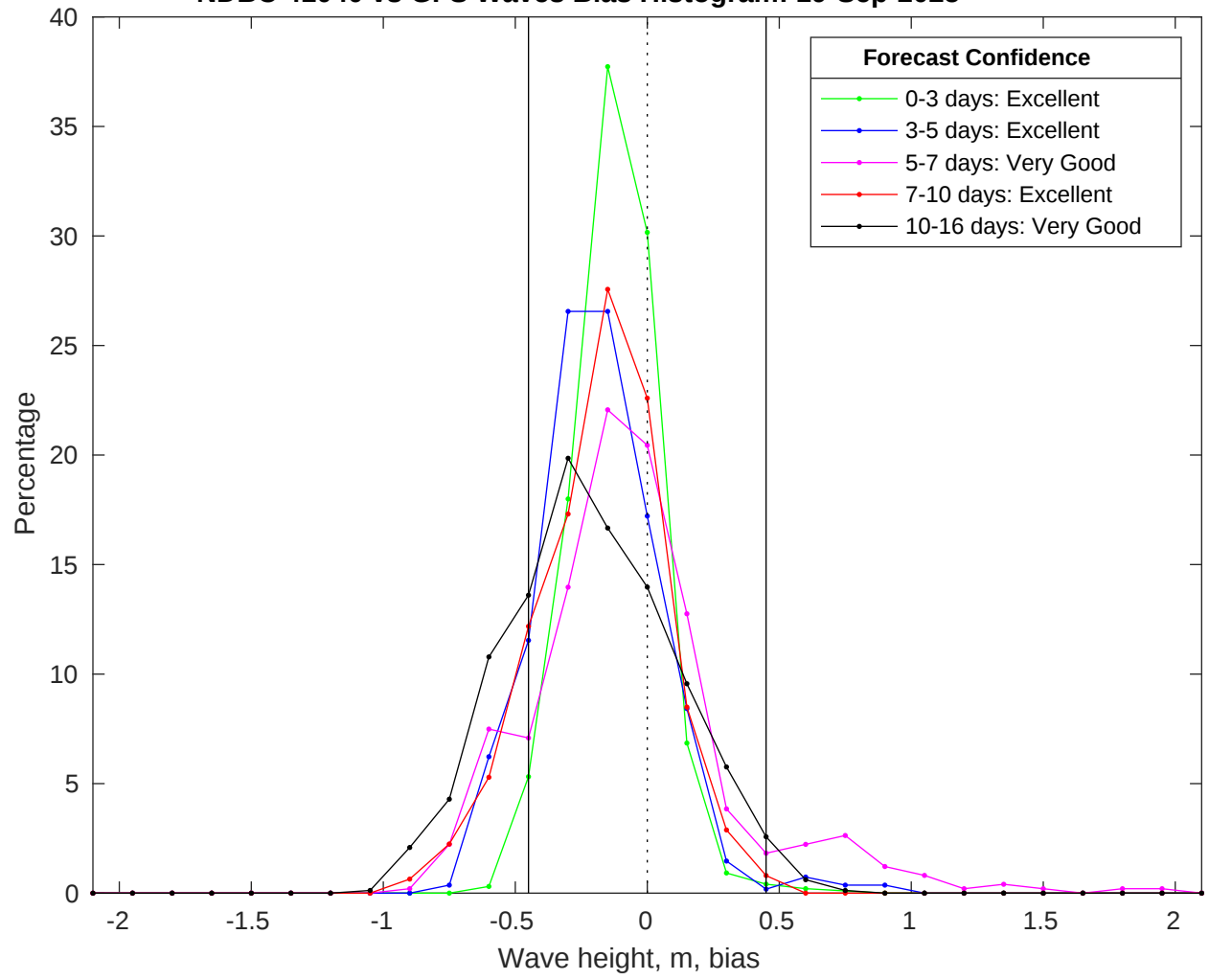
NDBC 41040 vs GFS Waves Bias Histogram: 19-Sep-2025
